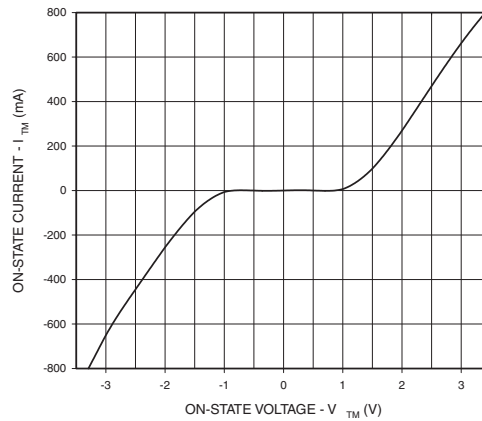
Fig. 2 On-State Characteristics
